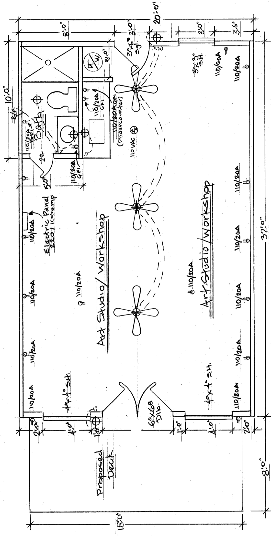
Floor Plan 640 sq. ft. 14"=1'-0"
