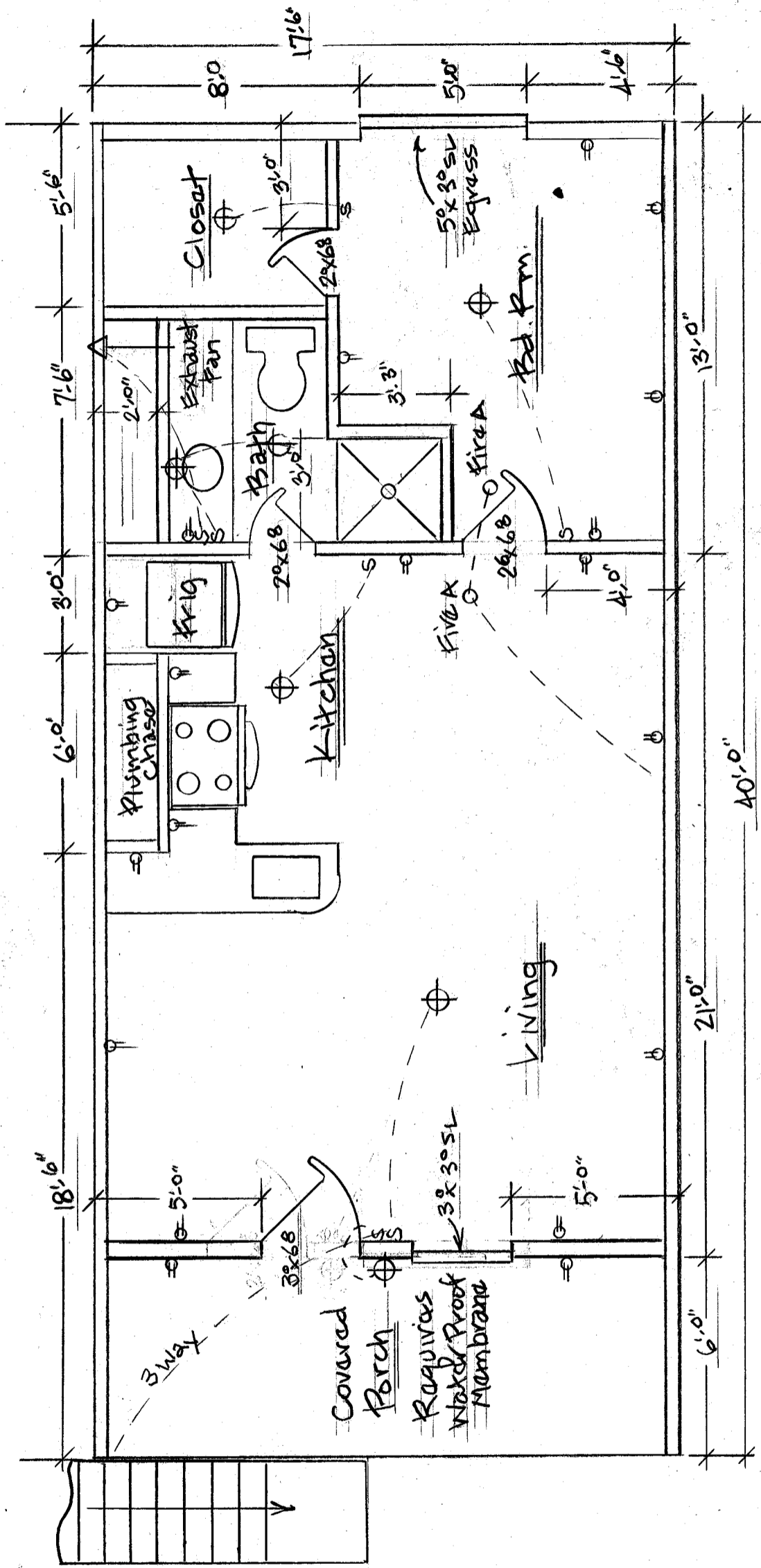
2nd Floor Plan 1/4" = 1'-0" 595 sq. ft.
