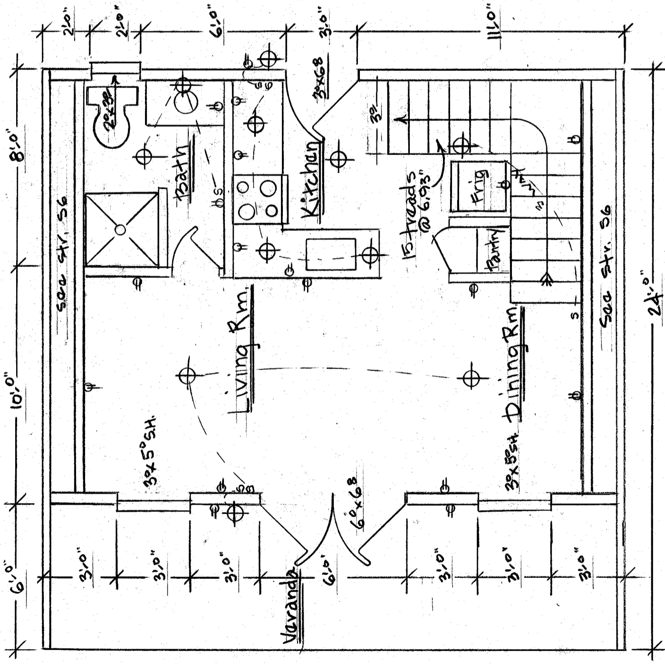
Main Floor Plan 1/4" = 1'-0" 434 sq. ft.
