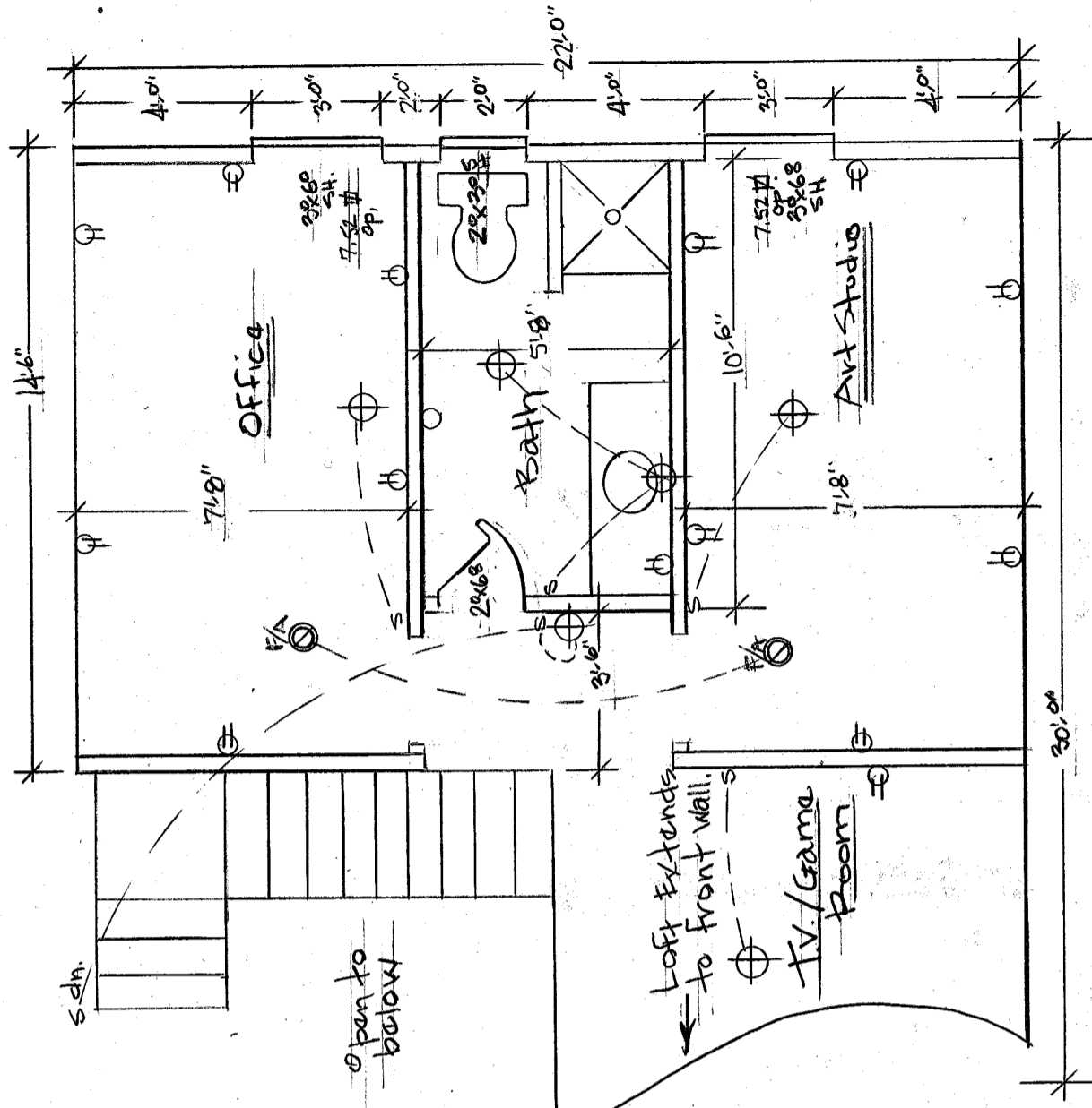
Second Floor Loft 14' = 14'0" ~ 238 sq. ft.
